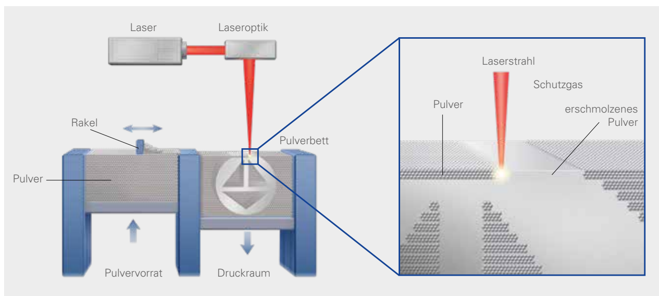
Powder Bed Fusion – Laser Beam (PBF-LB)
